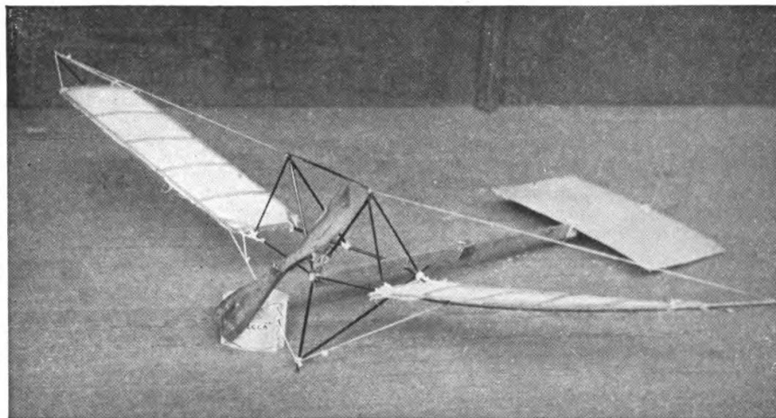
An interesting experiment in metal frame building by R. Fisher
