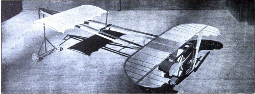
An efficient model, showing excellent construction, designed by John Caresi
