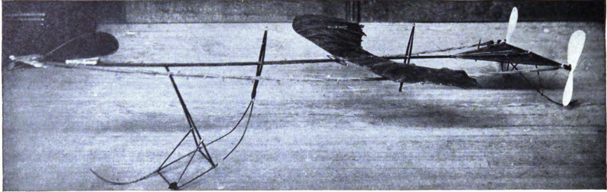
An American Fleming Williams built by C. McQueen
