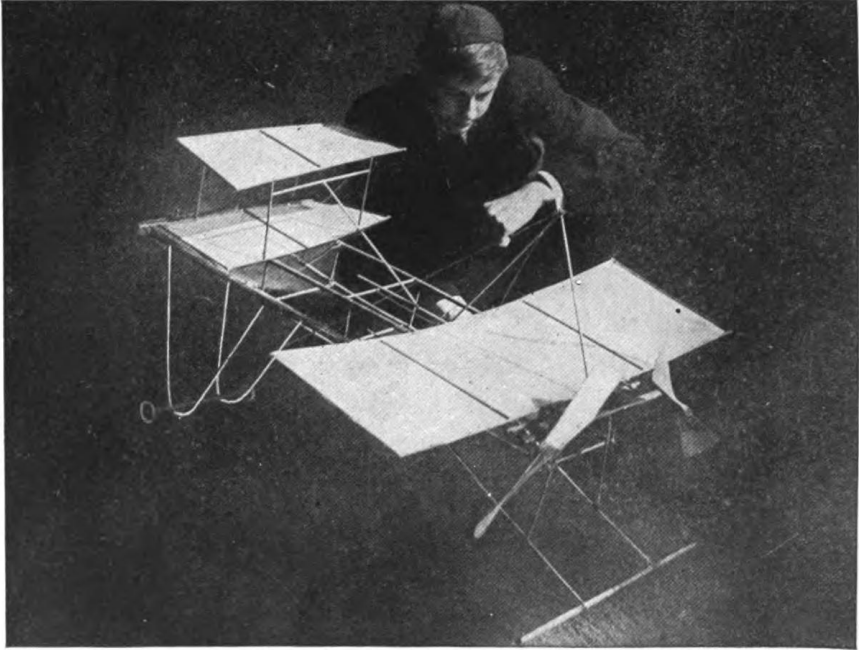
A successful model of 1910 built by E. G. Halpine. Note contrast in plane area
