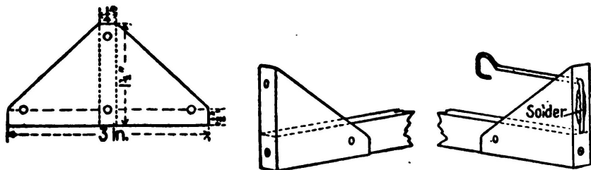
A Metal Motor Anchorage
