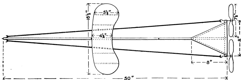
Working drawing of the Flemming Williams model
