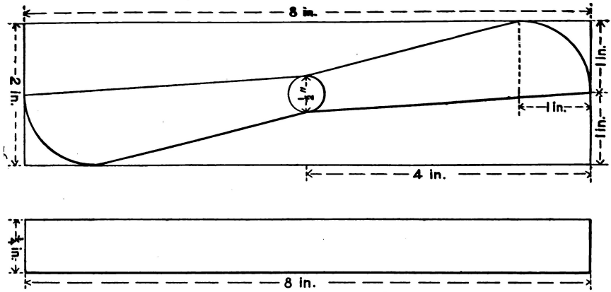
Diagram Showing How To Make A Propeller From A Wooden Blank
