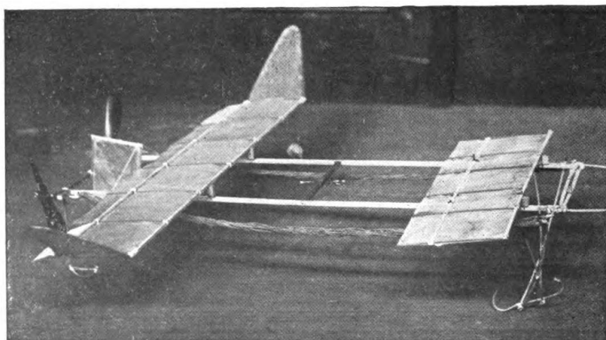
An early model built by Monroe Jacobs. Note the Ailerons.
