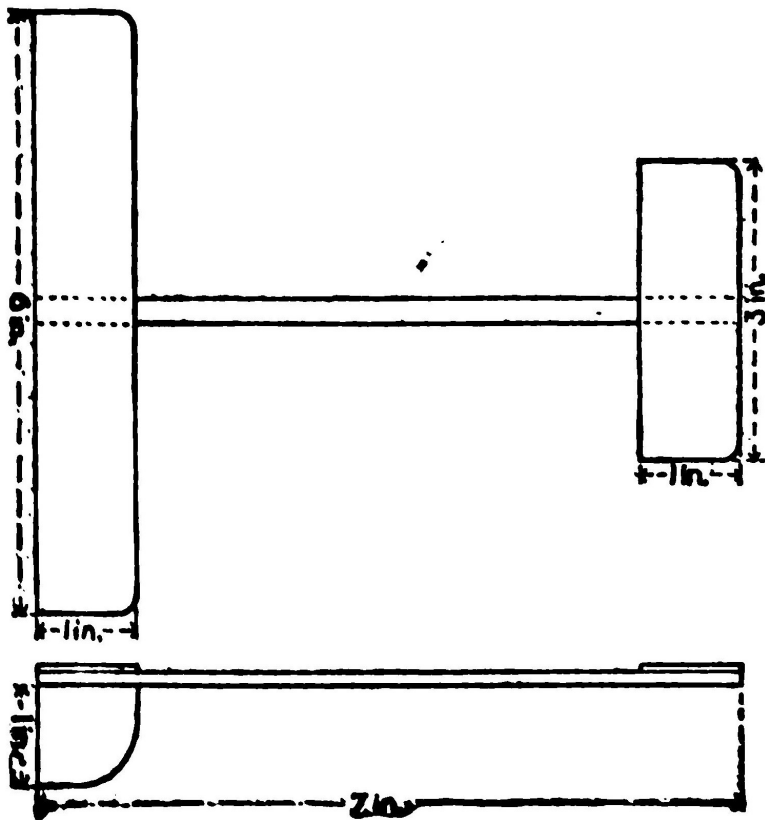
A Simple Model Glider
