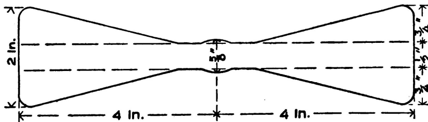
Langley Propeller Blade
