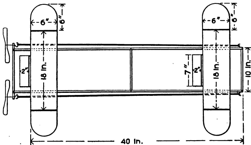
A Model With Adjustable Stabilizer.
