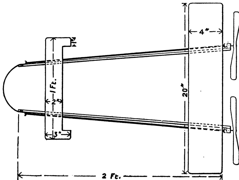
An Efficient Three-ounce Model.
