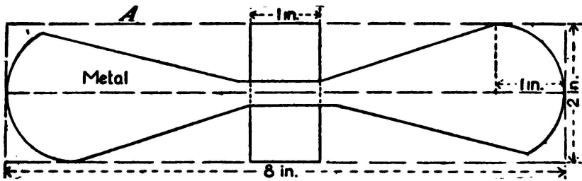
Design of Metal Propeller
