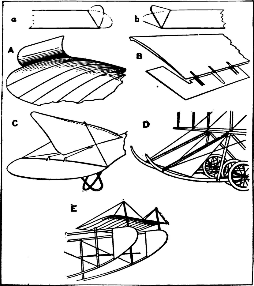
Various Steering Devices. "a" and "b," simple aileron forms. "A" novel fin on Vinet plane. "B" L-shaped aileron. "C" vertical rudder (Bleriot type). "D" "Blinkers," an effective rudder. "E" stability planes not unlike the runners of a sleigh.
