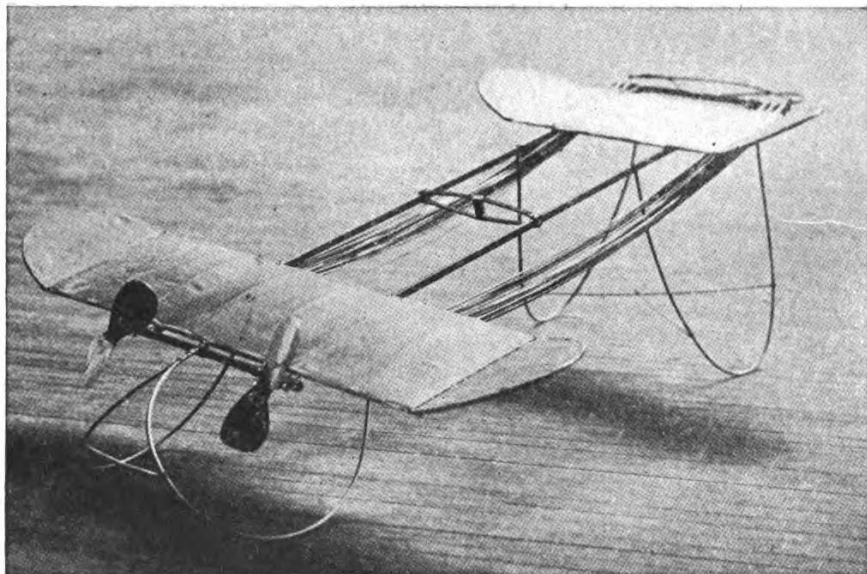
A geared model built by Leslie V. Robinson
