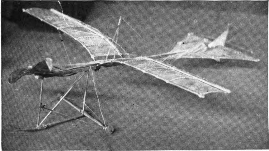
An interesting experiment in stability
