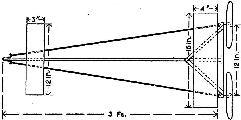
An All-metal Model Frame.
