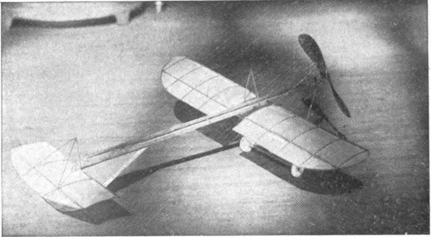
An excellent model, showing careful attention to details. Built by L. V. Brooks
