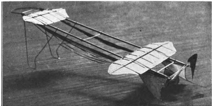
Long-distance model built by Percy Pierce.
