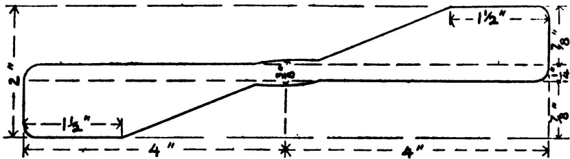
Wright Propeller Blade
