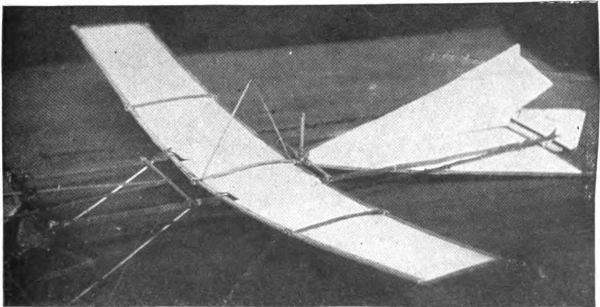
An early model built by E.G. Halpine
