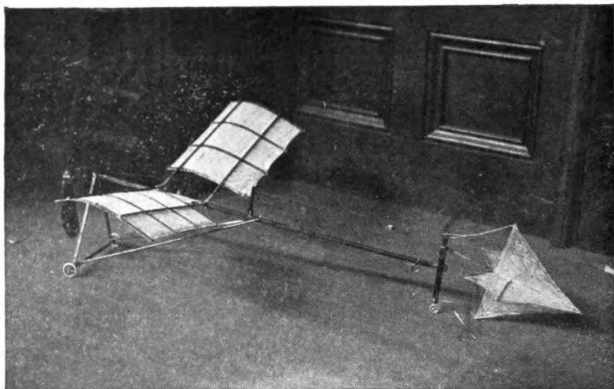
An interesting experiment in stability
